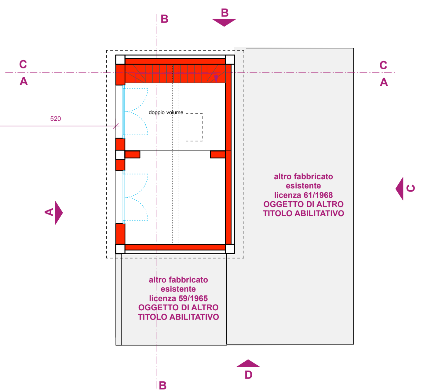
piano soppalco scala 1:100
